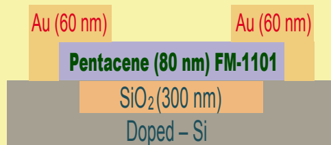
Schematic of OTFT Device
